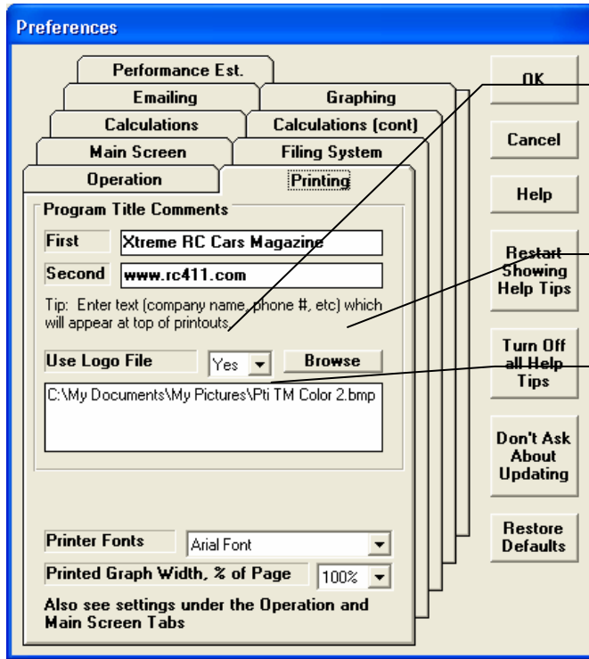
Figure A 7.5 Printing Company Logo (graphics file) on Graphs and Reports (Pro Version Only)
