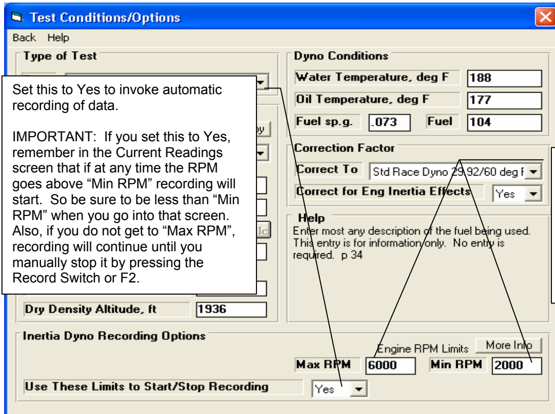
Figure 10.14 Setting Max/Min RPM for Automatic Recording in Test Conds Screen, Enterprise Edition Only
