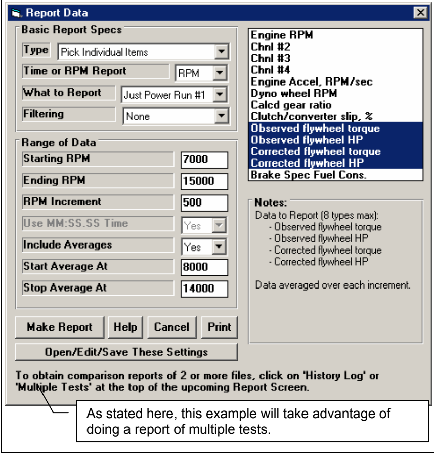
Figure 4.37 Report Options Menu
