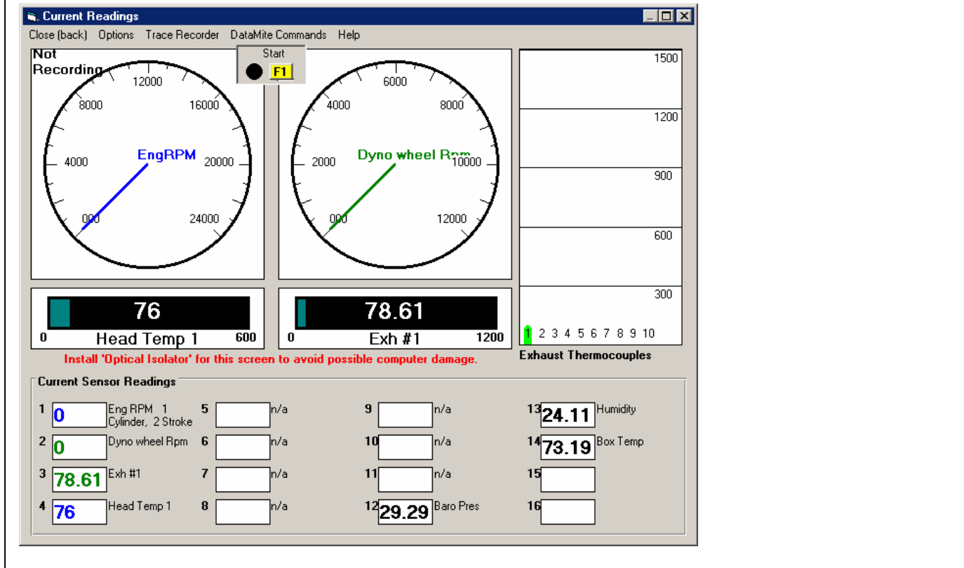
Figure 4.7 Checking Signals in Current Readings Screen (Engine Not Running)
