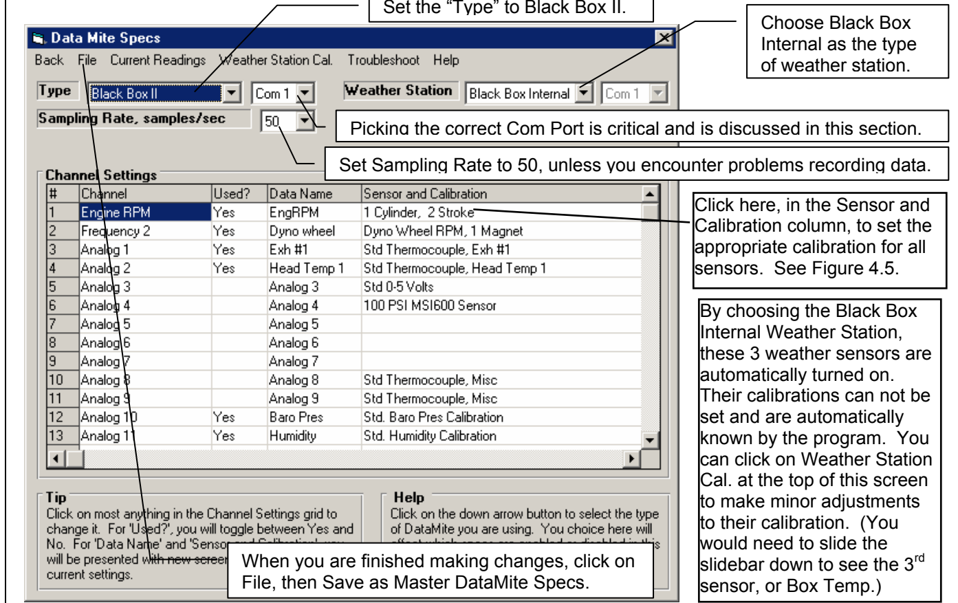
Figure 4.4 DataMite Specs Menu
