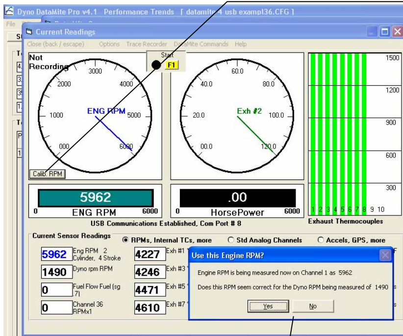
Figure A8.4 Test Conditions for Chassis Dynos, cont
