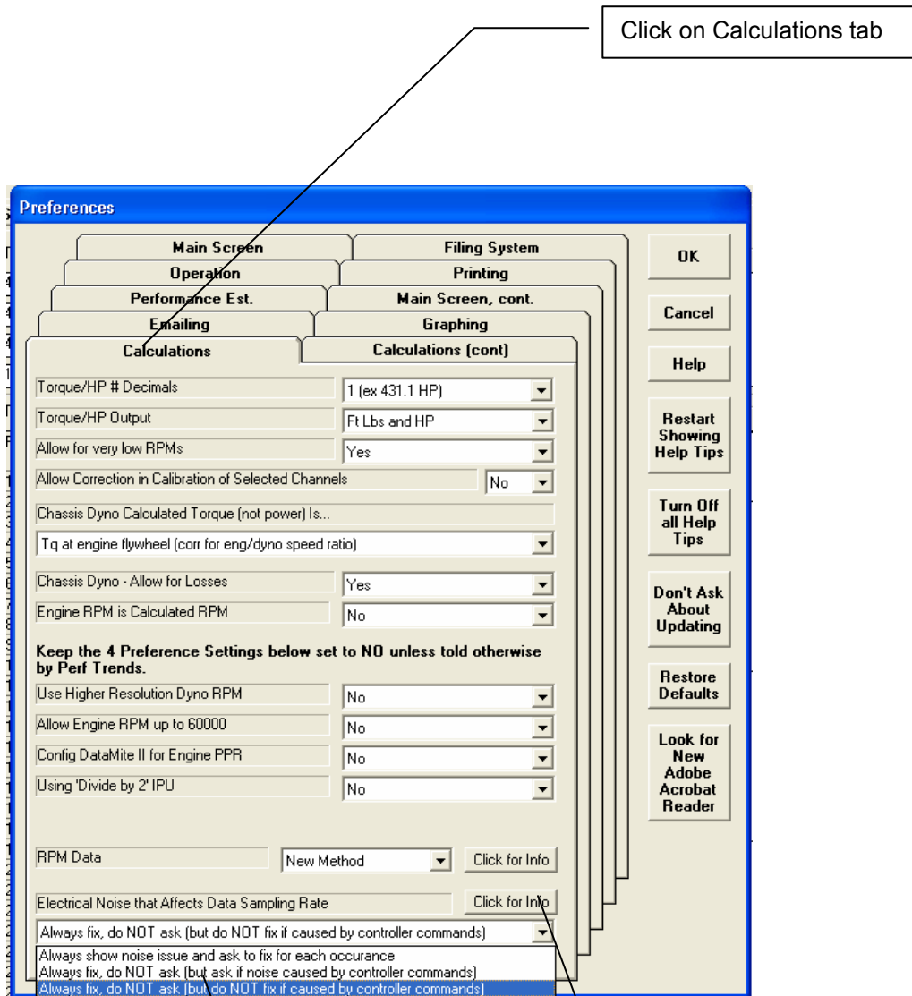
Figure 10.21 New Preference for Electrical Noise
