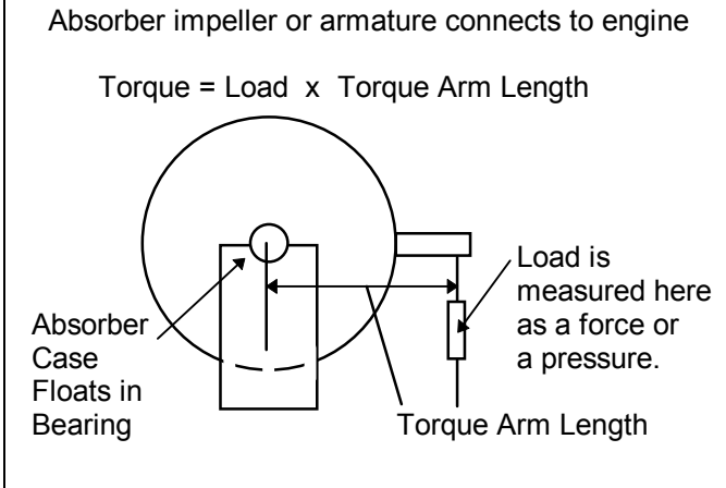
Figure A5.3 Torque Arm Type of Dyno
