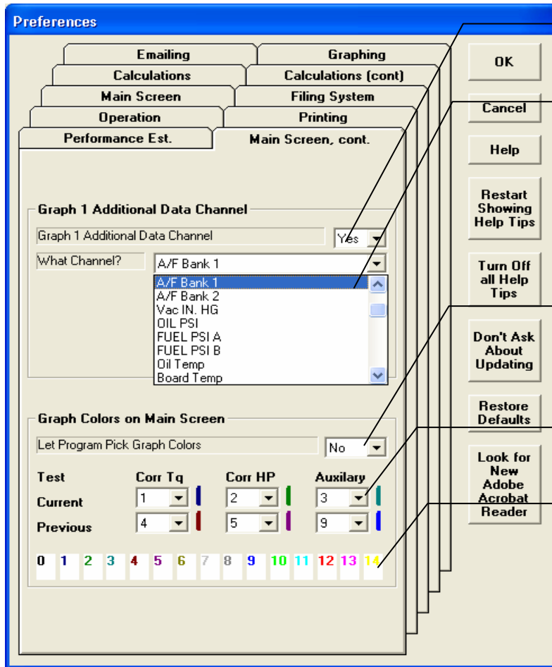
Figure 10.09 New Features for Graphs on Main Screen
