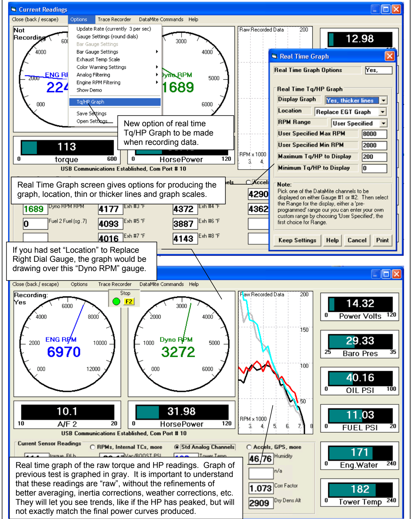
Figure A9.6 New 'Real Time' Graph, Enterprise Edition Only
